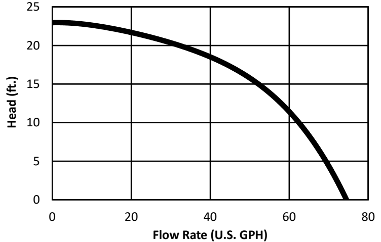
NT25-P18 Pump Curve
